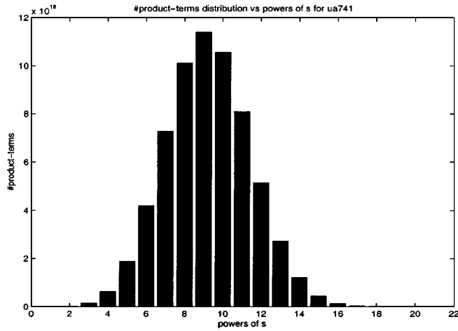
Fig. 13. Product-term distribution of \mu A741 over power of s for full symbol representation.
