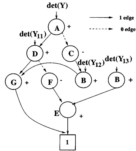
Fig. 10. DDD representing noise transfer functions.
