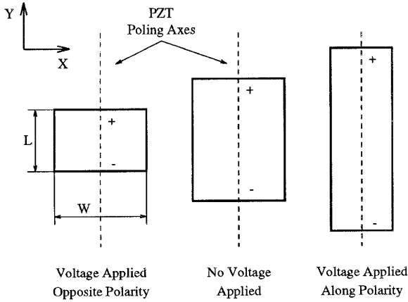
Fig. 1: PZT Expansion and Contraction
