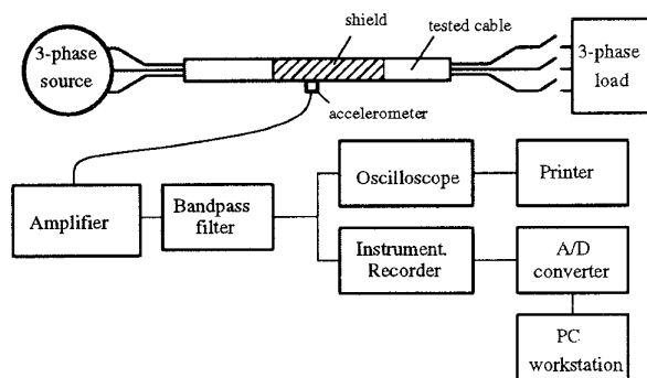
Fig. 2: Test Configuration
