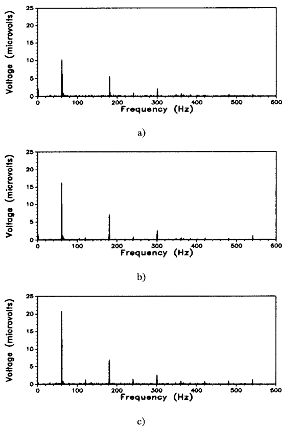
Fig. 3: Frequency spectrum of the sensor output signal when a shielded cable is a) non-energized, b) energized, c) energized and loaded.
