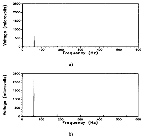
Fig. 4: Frequency spectrum of the sensor output signal when a non-shielded cable is a) non-energized, b) energized with and without load.
